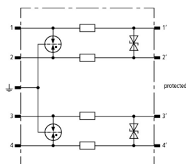
Basic circuit diagram BSP M4 BD 12
