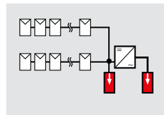
1 MPP / 2 Strings
