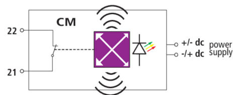
Basic circuit diagram DRC SCM XT
