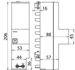
Dimension drawing DV ZP TNC 255
