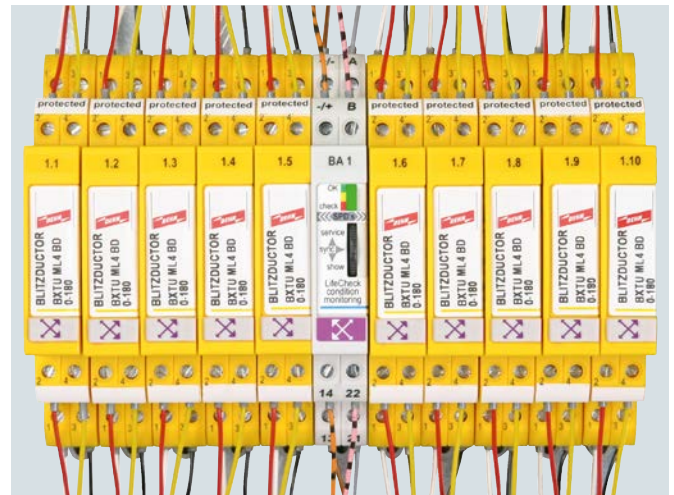
Installed DEHNrecord condition monitoring system
