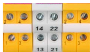
Floating remote signalling contact DRC MCM XT: break contact (21/22), make contact (13/14) DRC SCM XT: break contact (21/22)
