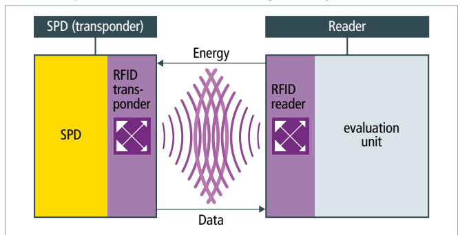
Communication principle between SPD and test device
