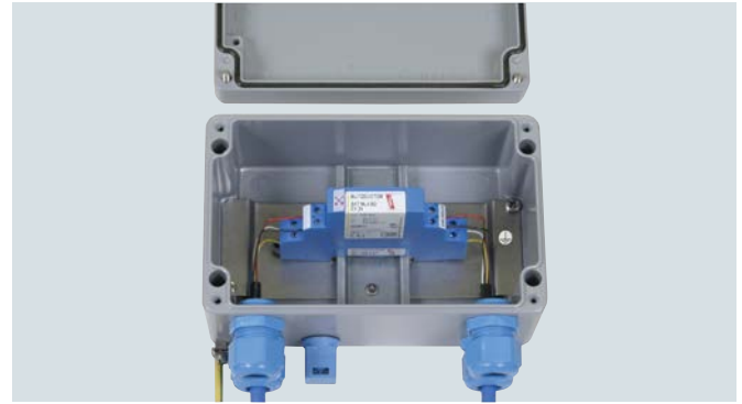
Pluggable and universal multipole surge arrester for use in intrinsically safe systems with integrated LifeCheck monitoring function.
