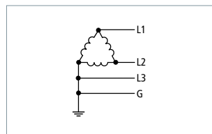
three-phase; 4 wire Delta "Grounded Corner"
