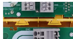
Side-by-side mounting of several devices thanks slide-in dovetail connections on the enclosures (DBX TC B 180).
